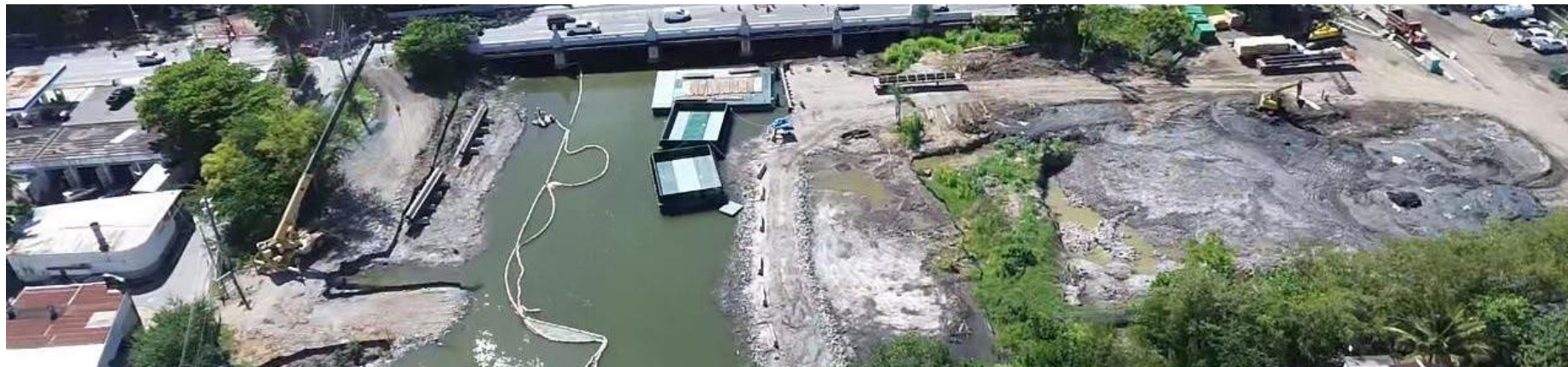
Caño Martín Peña Project CNT 2 – Western Bridges (Martin Peña, Tren Urbano, Ponce de Leon bridges) Scour Protection Construction
